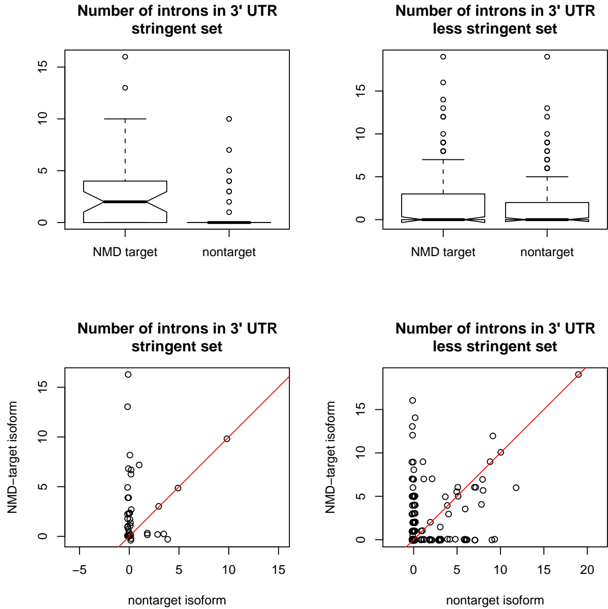
Figure S14. Number of introns in 3' UTR. As Figure S9 for the feature “number of introns in 3' UTR.” Both the bottom right and the bottom left scatterplots has been jittered.
