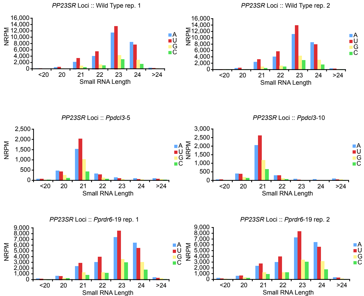
Figure S2. Distribution of small RNAs from Pp23SR loci by length and 5' nucleotide. Each graph represents the Pp23SR matched portion of the indicated small RNA library. A, U, G, and C refer to the identity of the 5' nucleotide. NRPM: Normalized reads per million.
