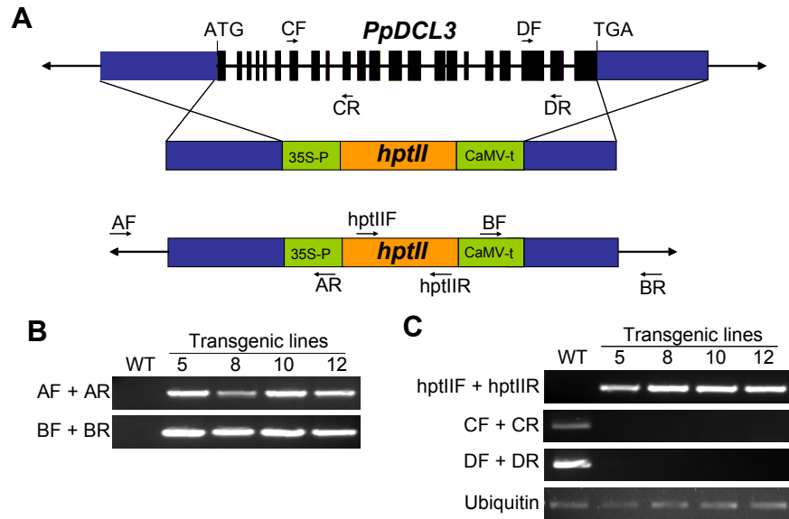
Figure S1. Targeted deletion of P. patens PpDCL3 . (A) Schematic of homologous recombination scheme. Labeled arrows indicate oligos used for PCR and RT-PCR analyses. Solid rectangles indicate exons, lines indicate introns. CaMV: Cauliflower Mosaic Virus, hptII : hygromycin phosphotransferase II gene. Not to scale. (B) PCR of genomic DNA using the indicated primer pairs. (C) RT-PCR analyses of gene expression using the indicated primer pairs.
