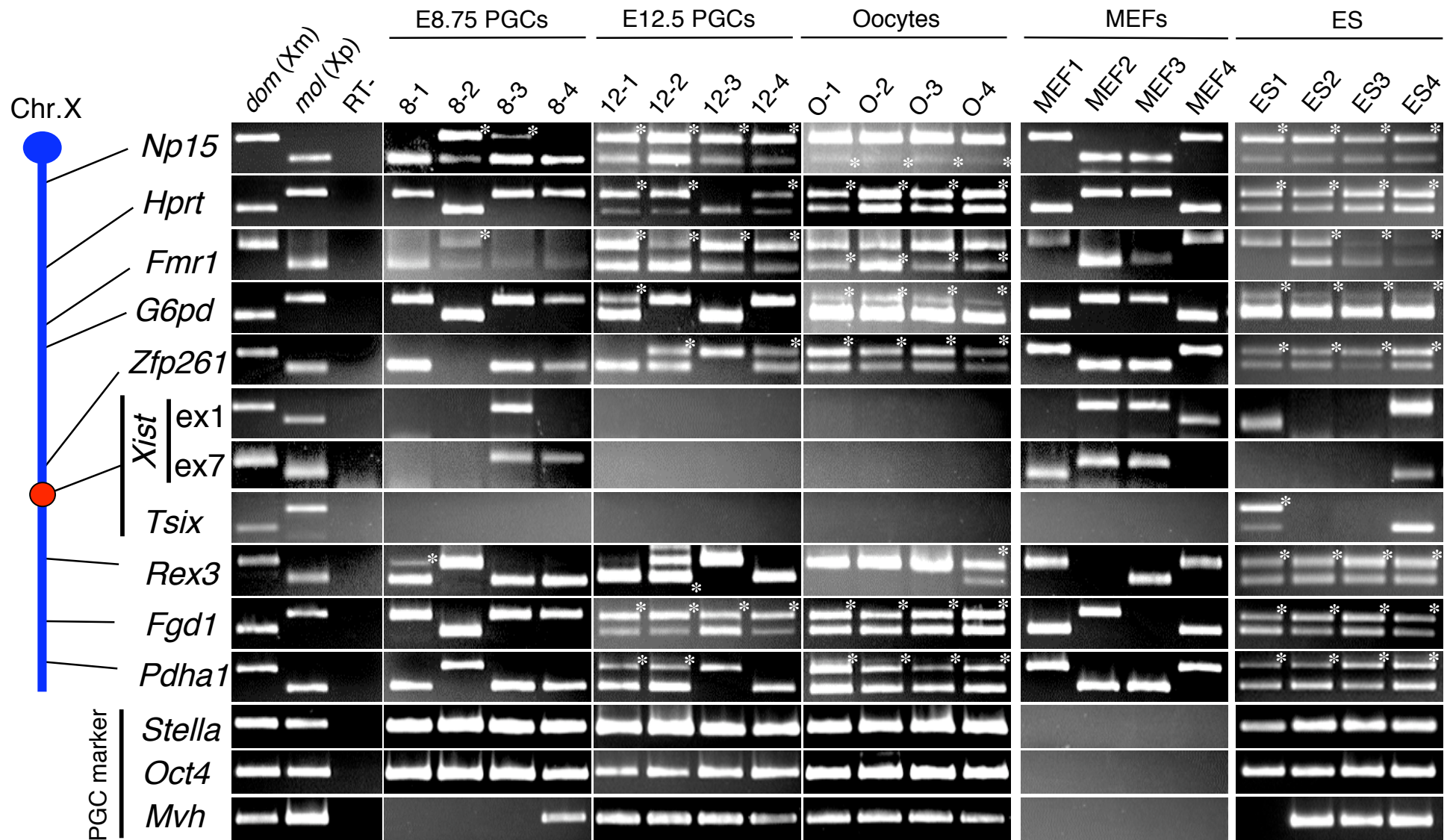
Figure. S4. Single-cell RT-PCR results of E8.75 PGCs, E12.5 PGCs, oocytes, MEFs, and ES cells. E8.75 and E12.5 PGCs were isolated from hybrid embryos generated from Oct4-GFP × MSM/Ms matings, and oocytes were from superovulated hybrid females. MEFs and ES cells were used as controls. Asterisks indicate biallelic expression.
