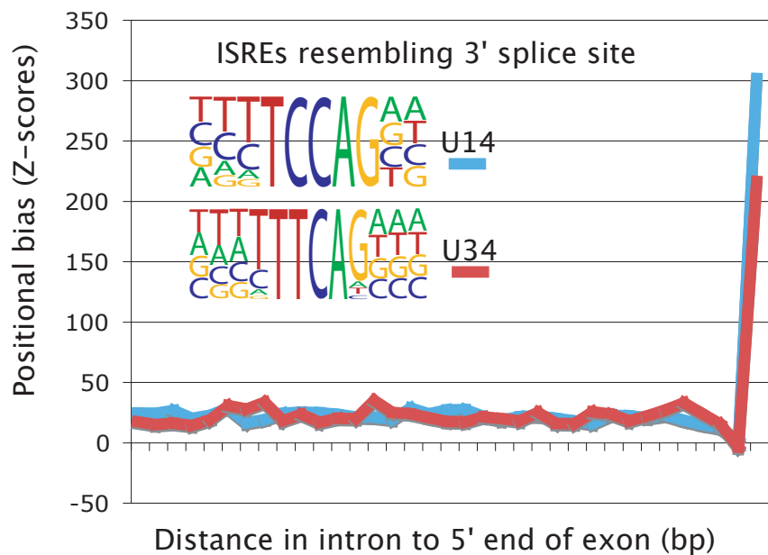
FIGURE S2. ISREs resembling canonical splice signals exhibit positional biases
