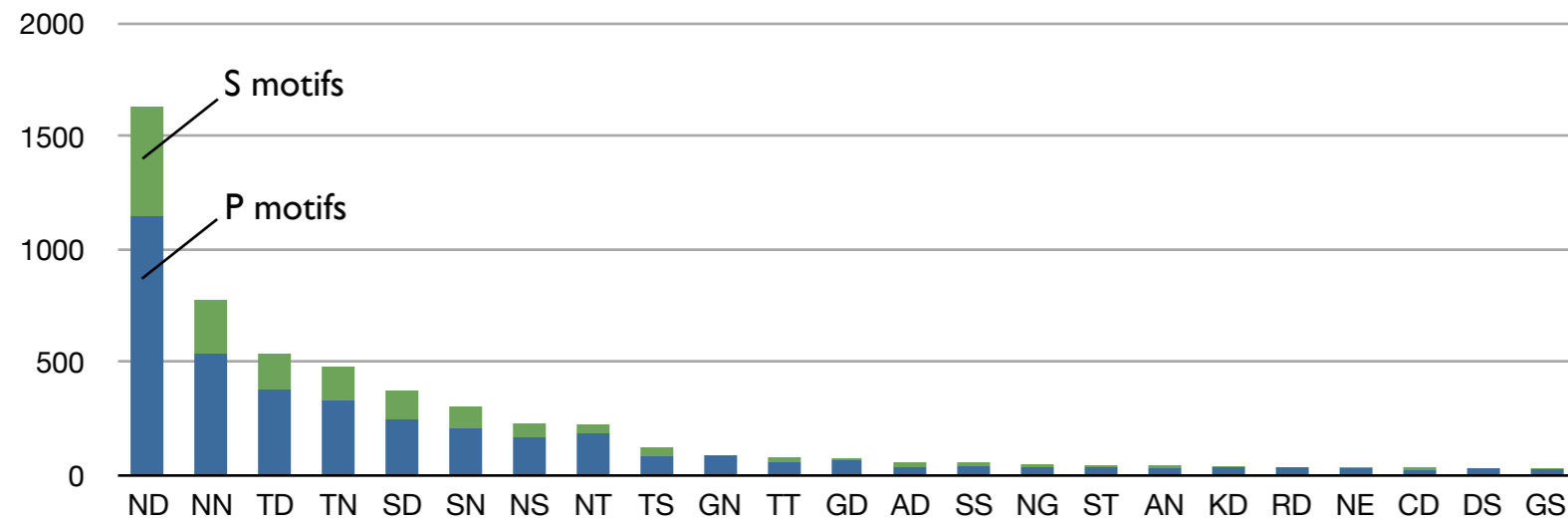
Figure S2. Frequency of 6,1' combinations in Arabidopsis PPR proteins. The most frequent combinations are shown (all those observed more than 30 times). Only tandem pairs of motifs (5362 in total) were considered in this analysis, where the first motif was either a P or S motif. Combinations observed in P motifs are shown in blue, those in S motifs in green.
