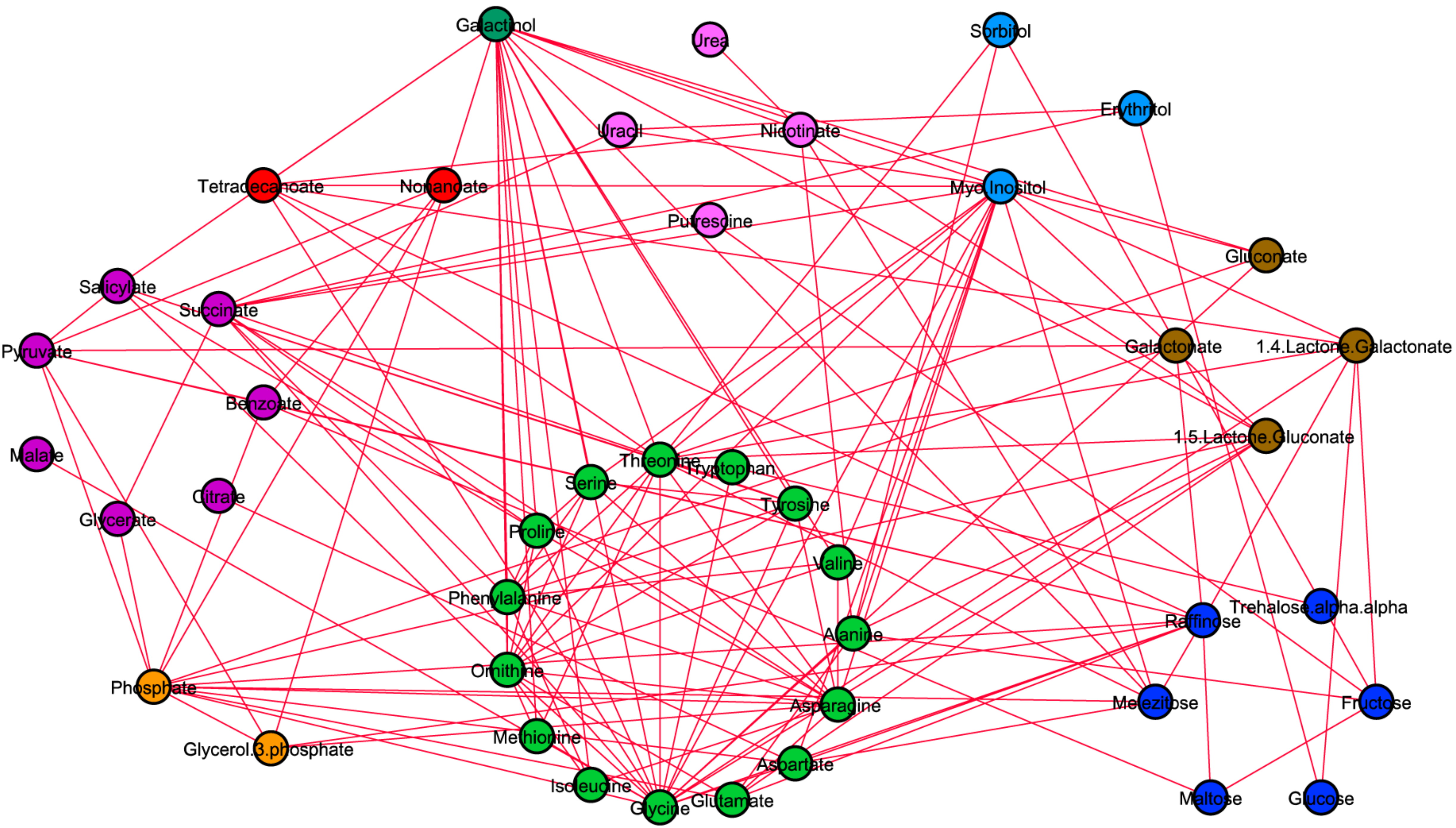
Seed harvests 2004-2005 conserved correlations - compound class-connectivity view r \geq 0.3 , p \leq 0.01
