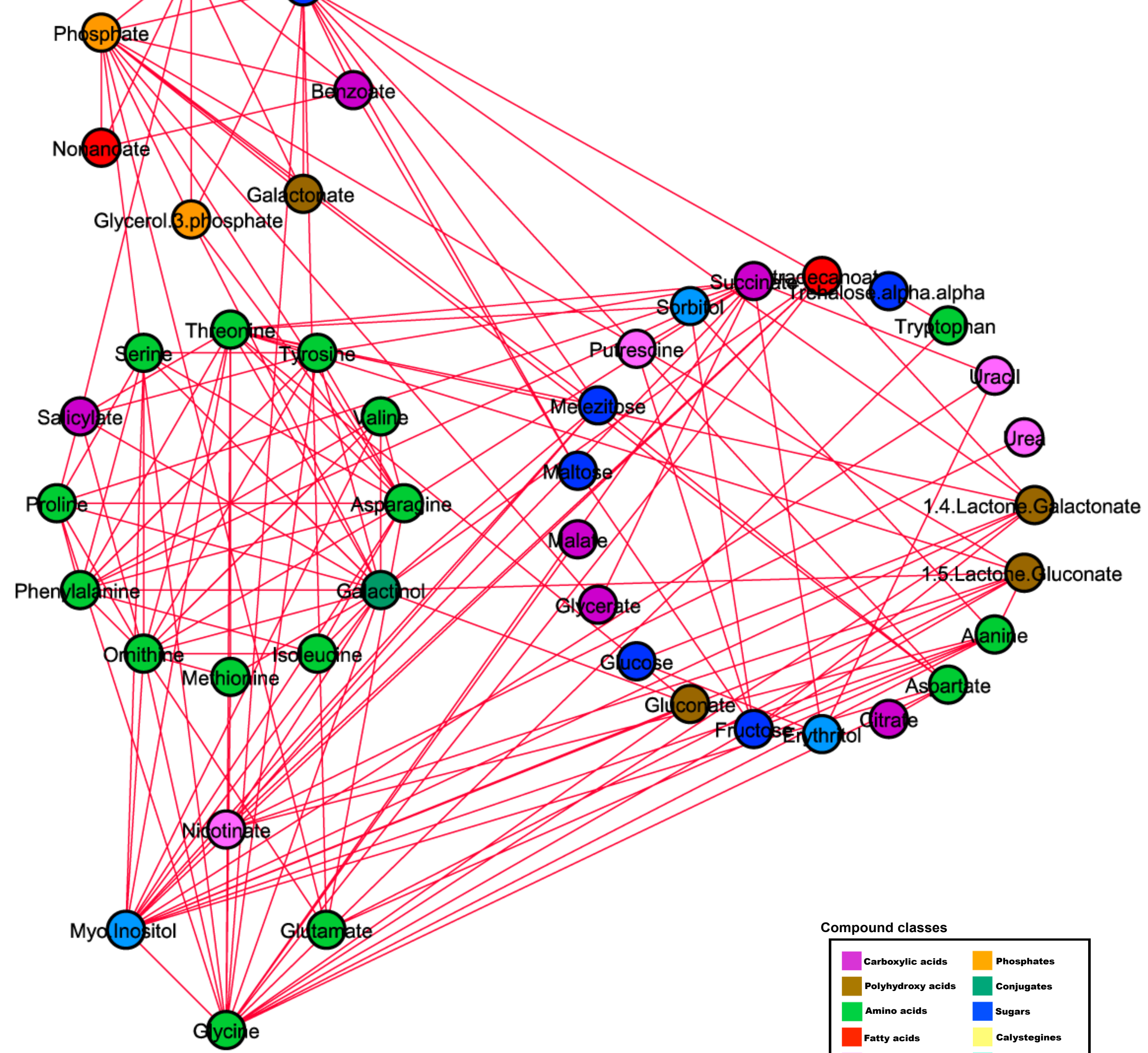
Seed harvests 2004-2005 conserved correlations - cluster view r \geq 0.3 , p \leq 0.01
