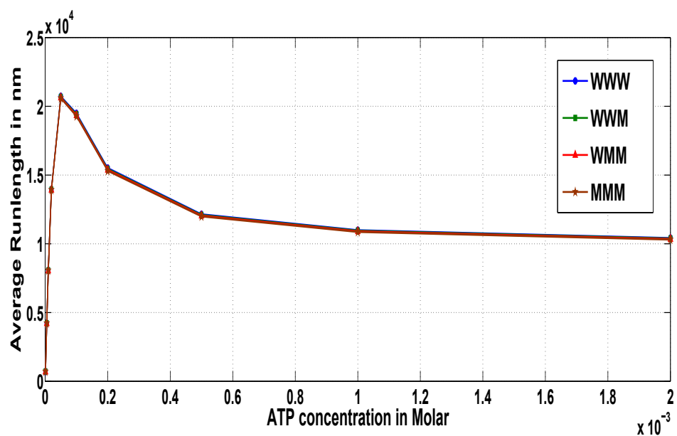
Figure 1: Effect of ATP concentration on average runlength for 3-motor ensembles WWW, WWM, WMM and MMM against load force of 0.2 \text{ pN}
