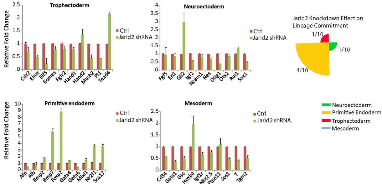
Figure S5. Expression measurements of lineage specification markers after knockdowns in mESCs
