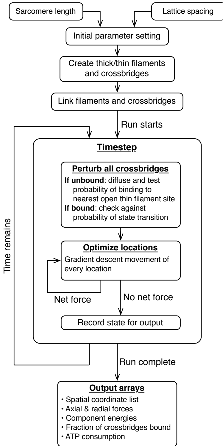
Figure S2: Model code structure and information flow. A diagrammatic representation of the steps that occur during a simulation, and which produce the measured forces and energies.
