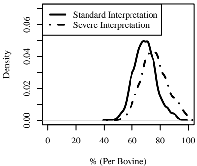
Occult Period T_O
