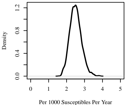
Infectious Pressure \chi_1
