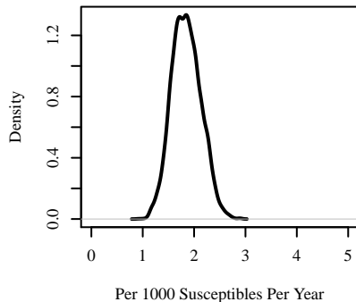
Infectious Pressure \chi_2
