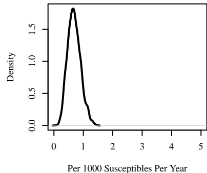
Infectious Pressure \chi_4
