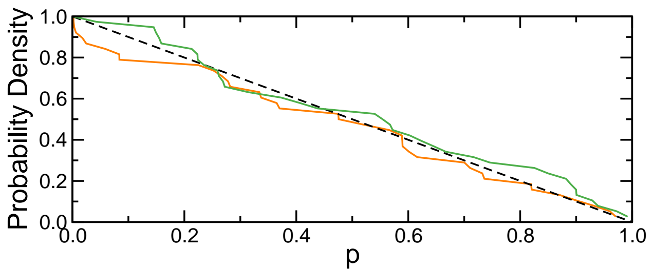
Figure S3: Brood sizes are normally distributed. Empirical distribution of p-values (orange), is consistent with the theoretical uniform distribution (black dashed). To confirm this, we generated 10,000 distributions consistent with the hypothesis that the empirical distribution is uniform. One of these is shown for illustration (green). Details of the experimental procedure are given in Supplemental Text.
