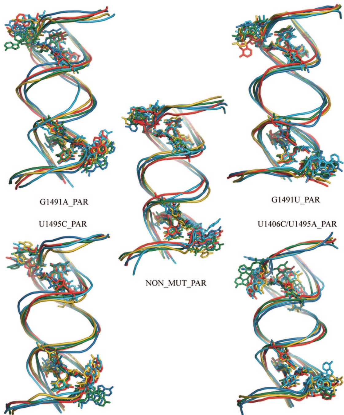
Figure S7: Representative structures of the clusters for different MD simulations of the A-site in the complex with paromomycin , superposed with regard to phosphorous atoms. Structures from each cluster are colored differently: 1 — green, 2 — blue, 3 — red, 4 — yellow, 5 — cyan (see Table S1 for the cluster sizes). Paromomycin and A1492, A1493 and A1408 are shown in atomic detail.
