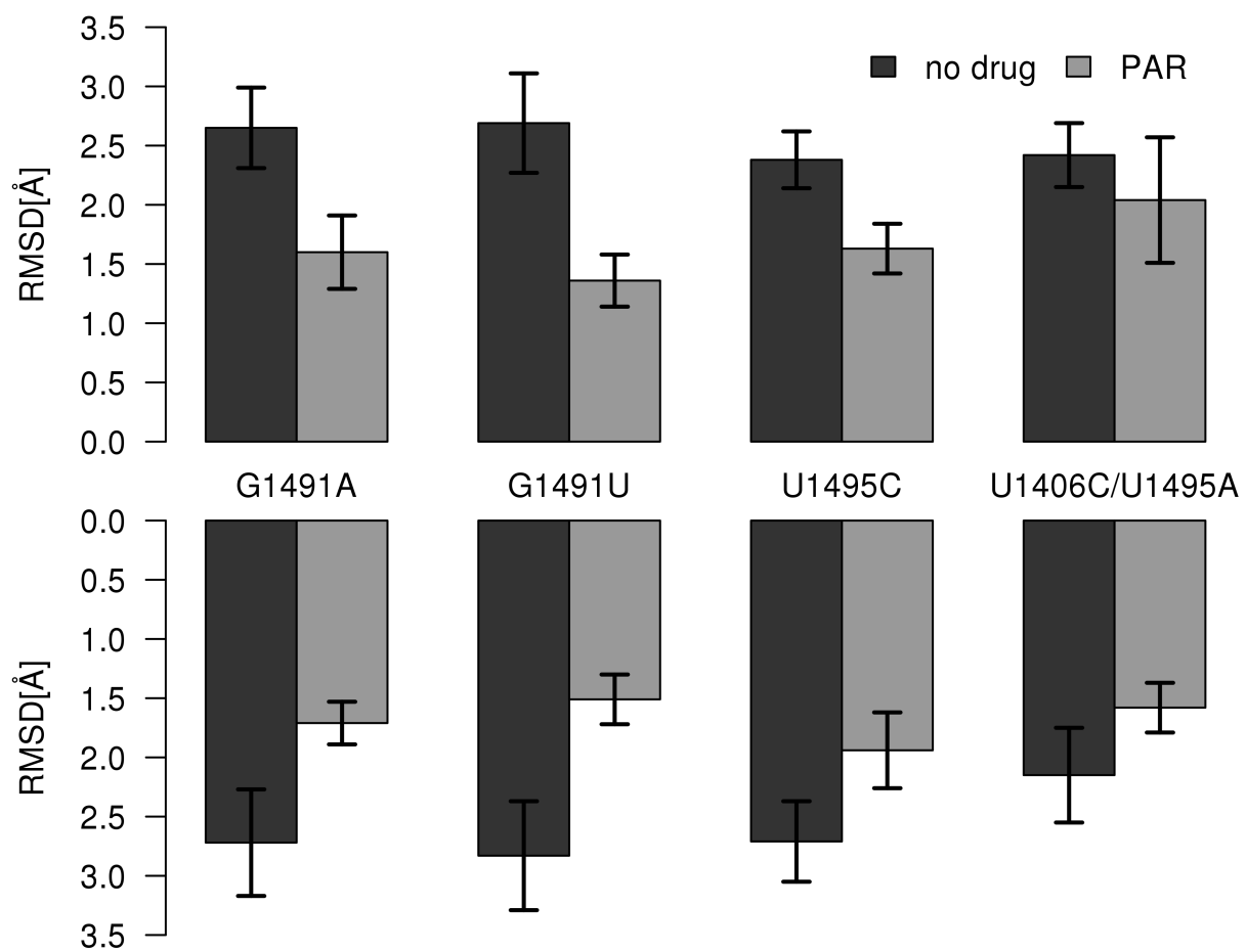
Figure S2: Average RMSD [Ångstrom] with their standard deviations; two graphs depict RMSD for two A-sites.
