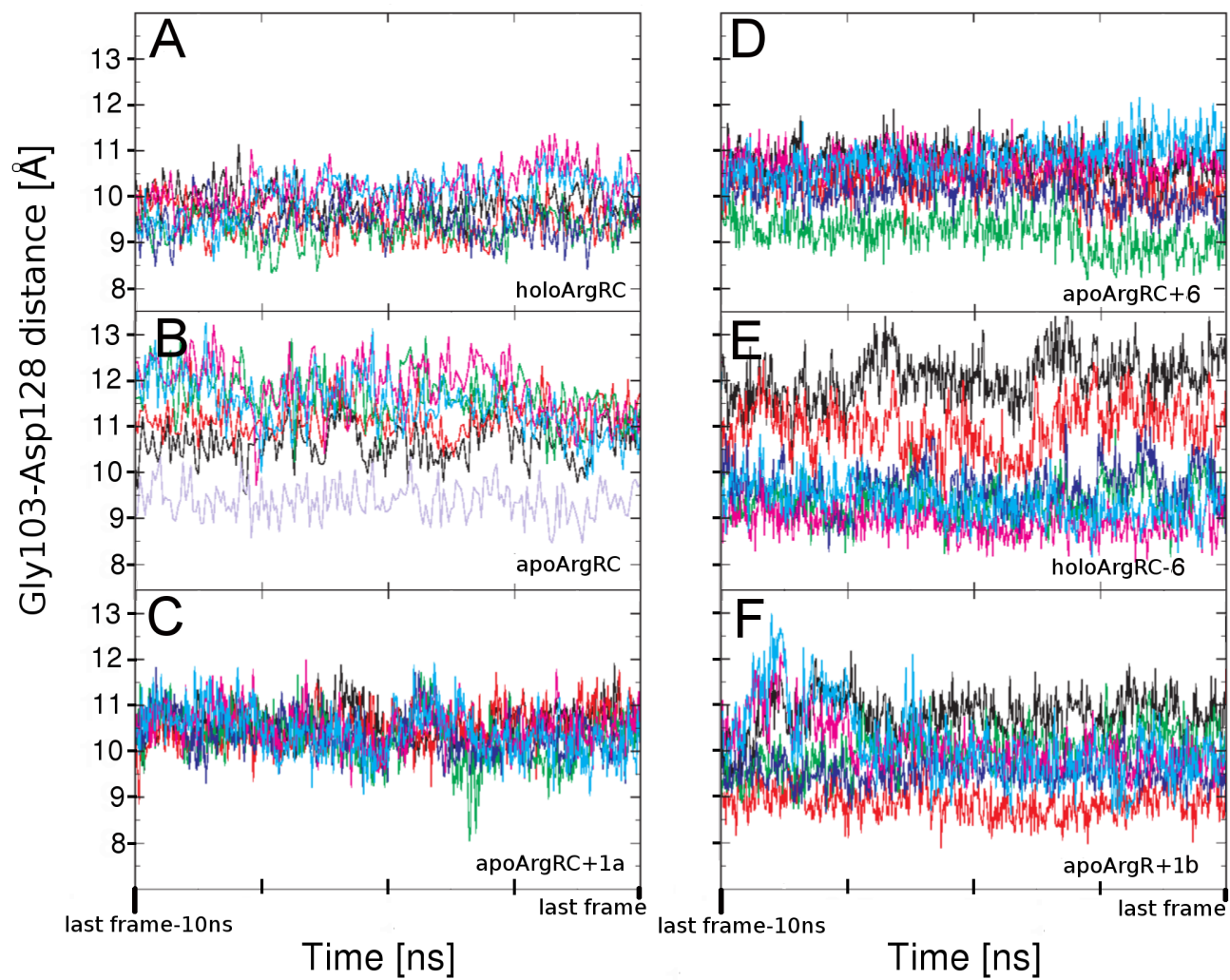
Figure S2. Gly103-Asp128 distances.
