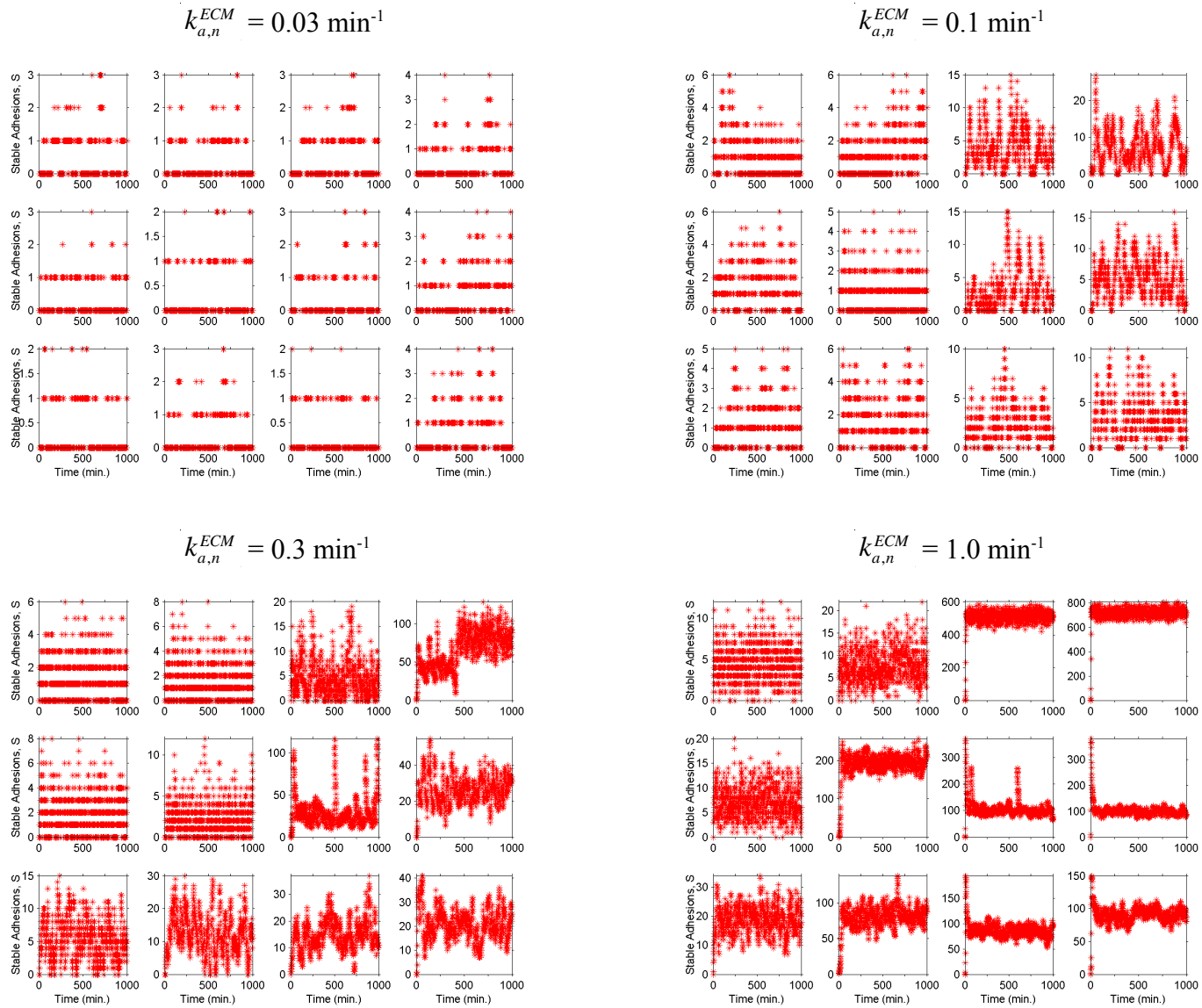
Fig. S2 C. Molecule number scaling: N^* = 10
