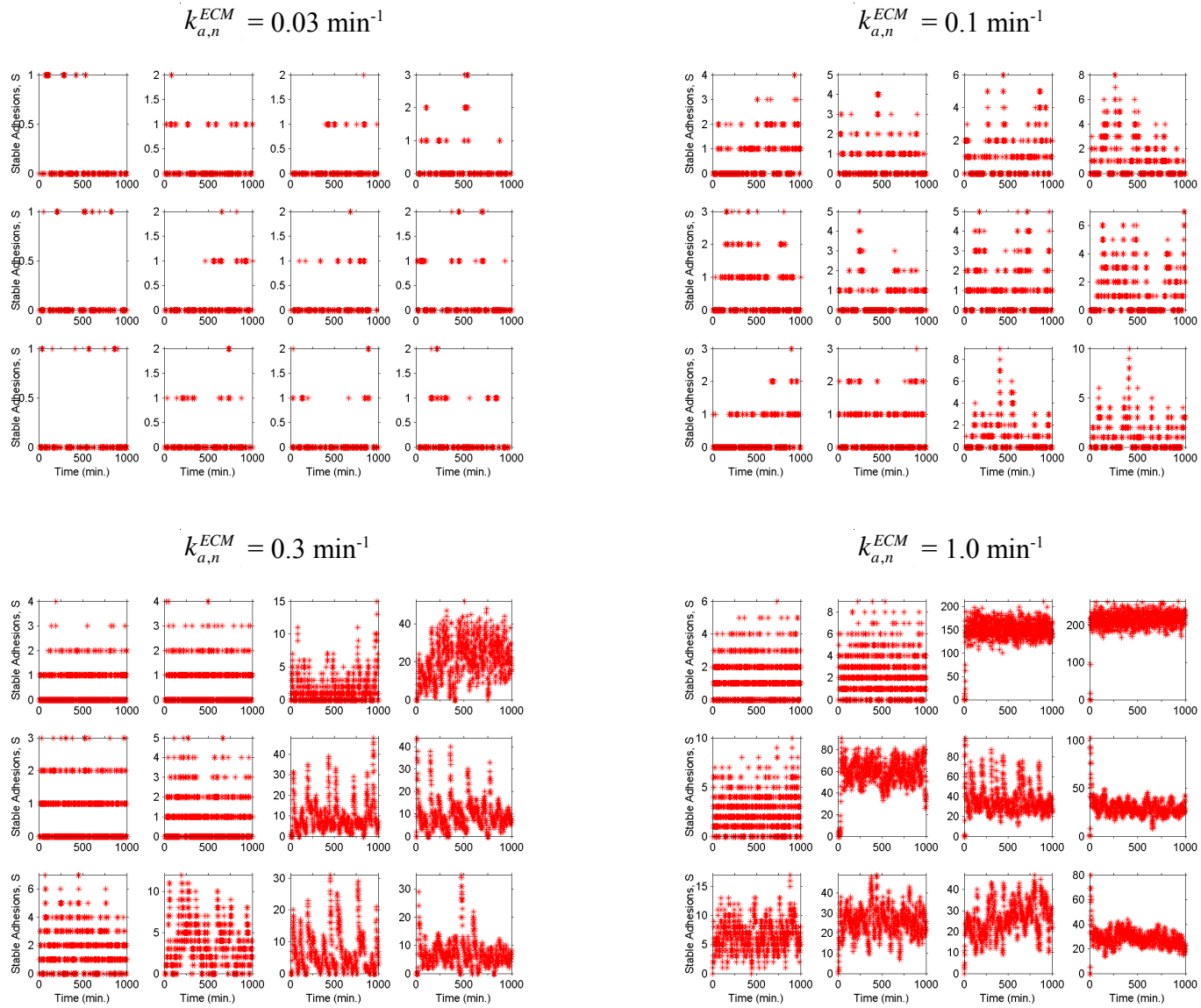
Fig. S2 B. Molecule number scaling: N^* = 3
