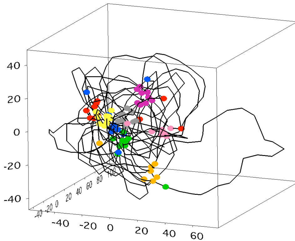
Figure 5: Typical spatial conformation for both the polymer and the interacting sites in a steady state for a random positioning of the sites. Note that several sites do not belong to any focus. Naked DNA, N_t = 8 , d^* = 6 nm, L = 8 \mu m and \lambda = 2l_p .
