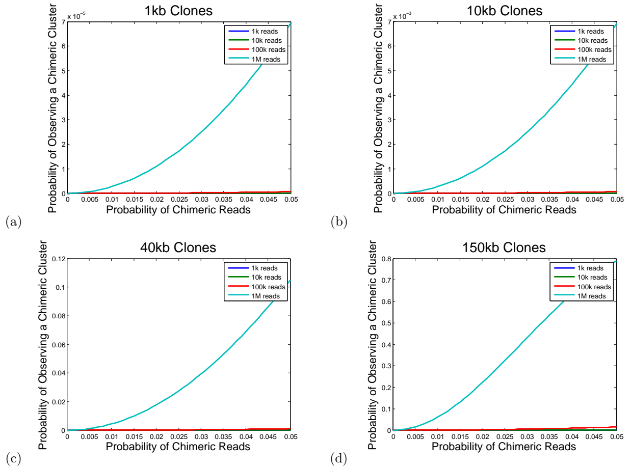
Figure 8: Effect of chimeric clones. Probability of observing at least one chimeric cluster vs. the percent of chimeric clones under equal number of paired reads indicates lower chimerism for smaller clones. (a) 1kb clones, (b) 10kb clones, (c) 40kb clones, and (d) 150kb clones.
