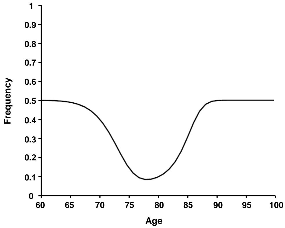
FIGURE 3S: Trend of Genotypic Frequency in simulated Age-structured population
