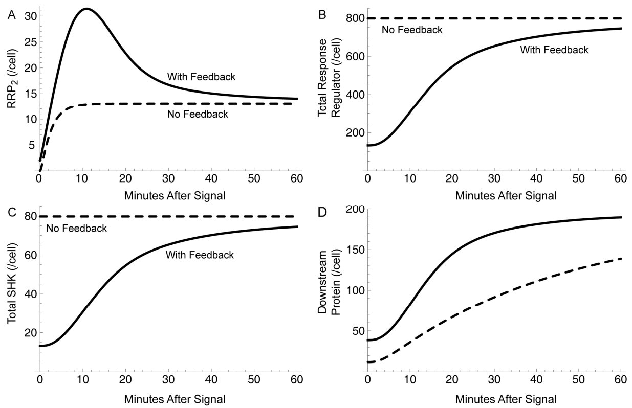
Figure S1. Characteristics of two-component system model calibrated to resemble Salmonella PhoPQ.
