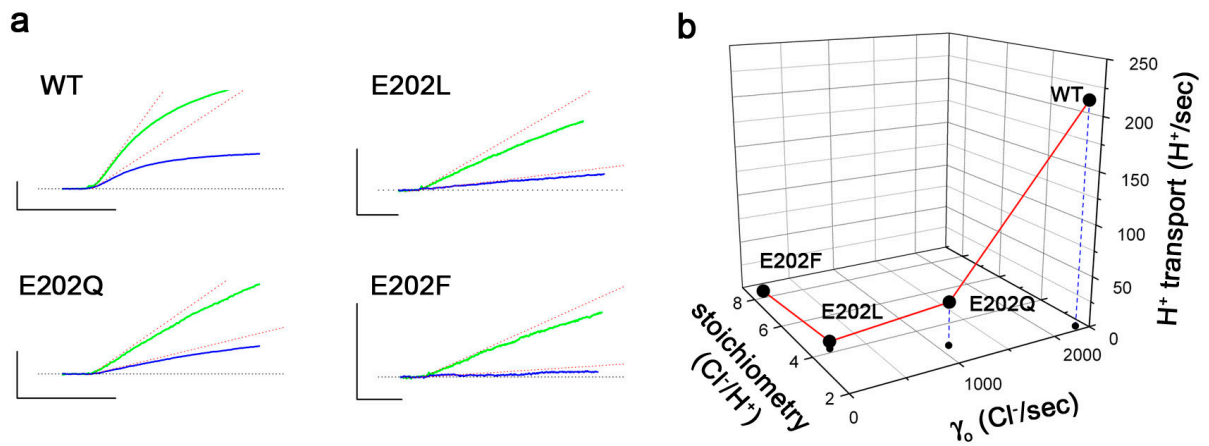
Figure S6. Coupling of Cl - /H + transport in E202 mutant transporters.
