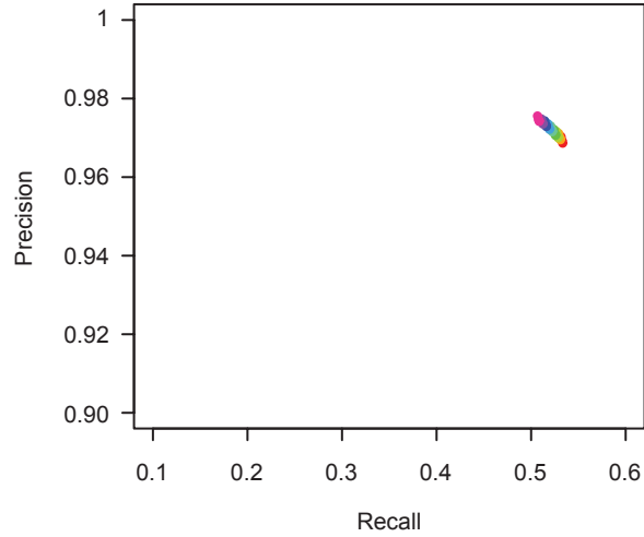
C Human Brain 50-mers, paired-end Junction read coverage \geq 1
