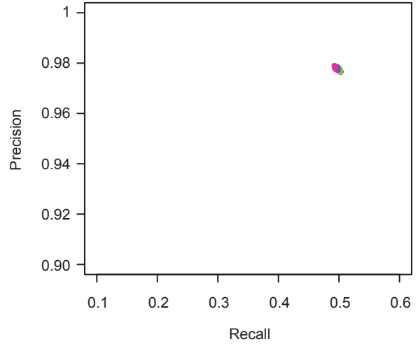
D Human Brain 50-mers, paired-end Junction read coverage \geq 2
