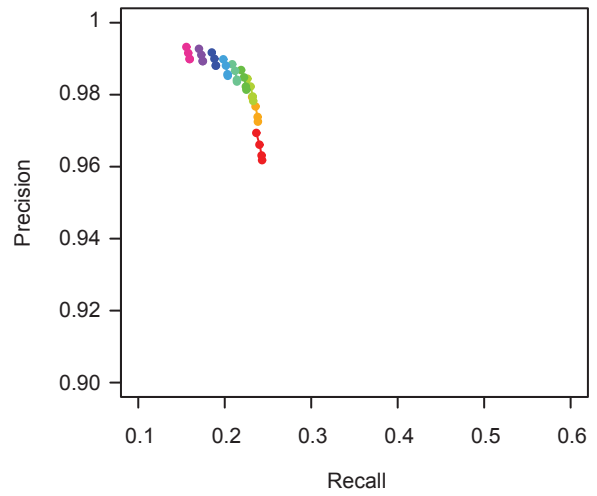
B Human Brain 32-mers, single-end Junction read coverage \geq 2
