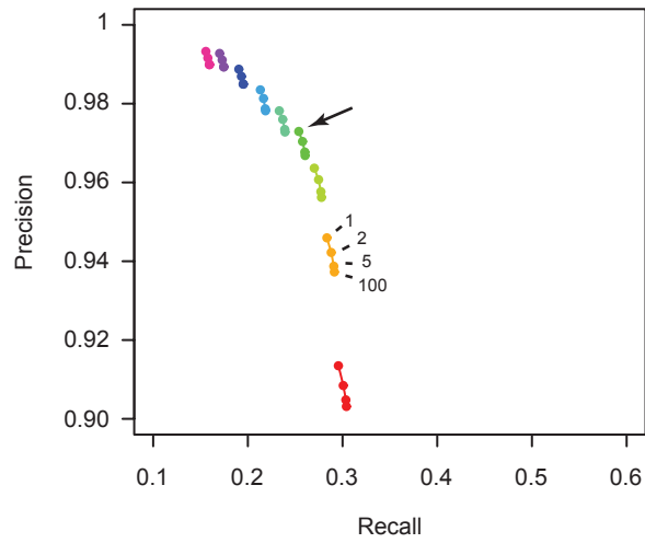
A Human Brain 32-mers, single-end Junction read coverage \geq 1
