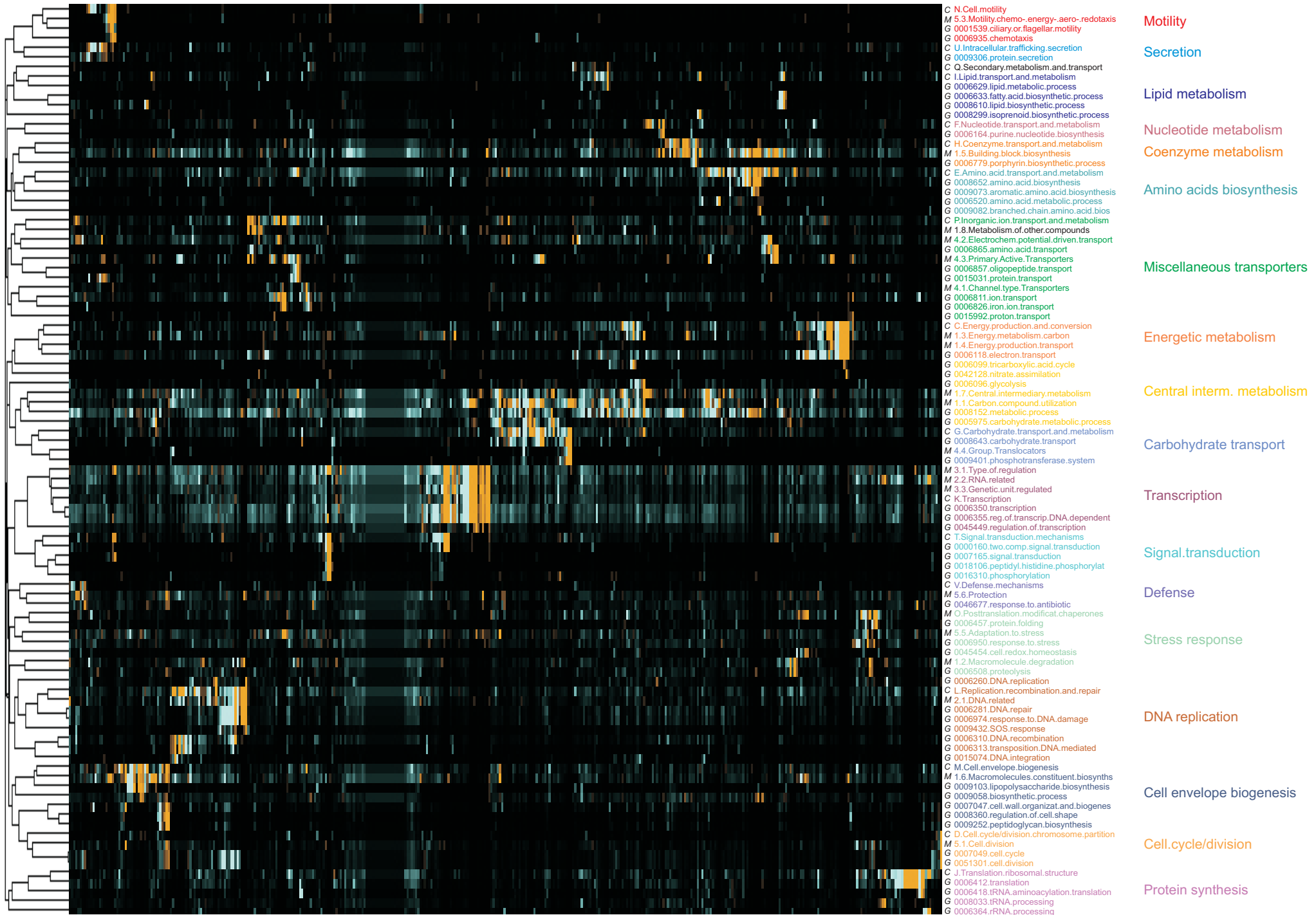
FigureS5 – Clustered annotation terms and functional neighborhoods.
