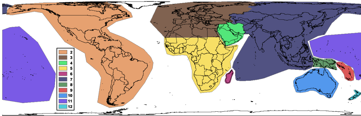
Fig. S1. Data sources for geographic range maps. A map illustrating the core references used for geographic sub-regions. Select additional sources such as island species lists were used.
