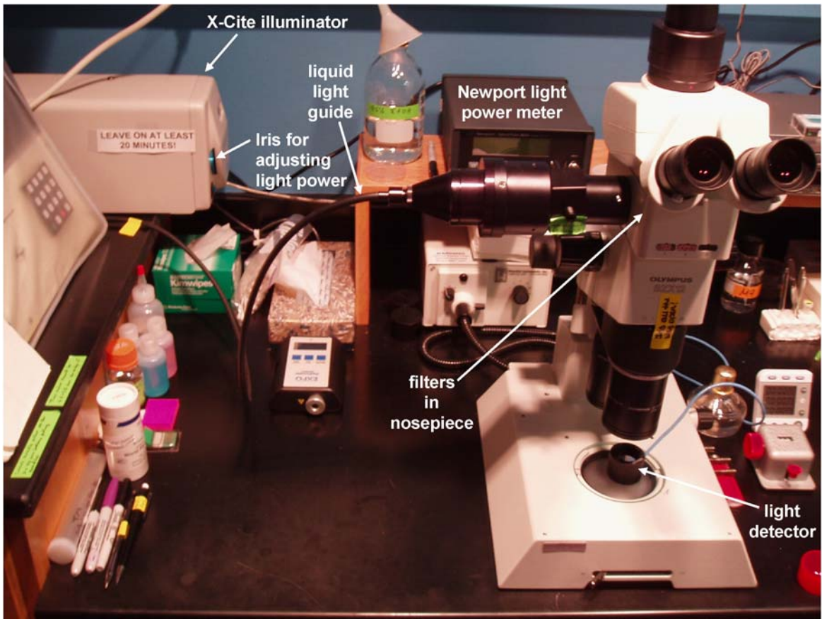
Figure S7. Method for Measuring and Controlling Light Power through a Stereomicroscope Objective
