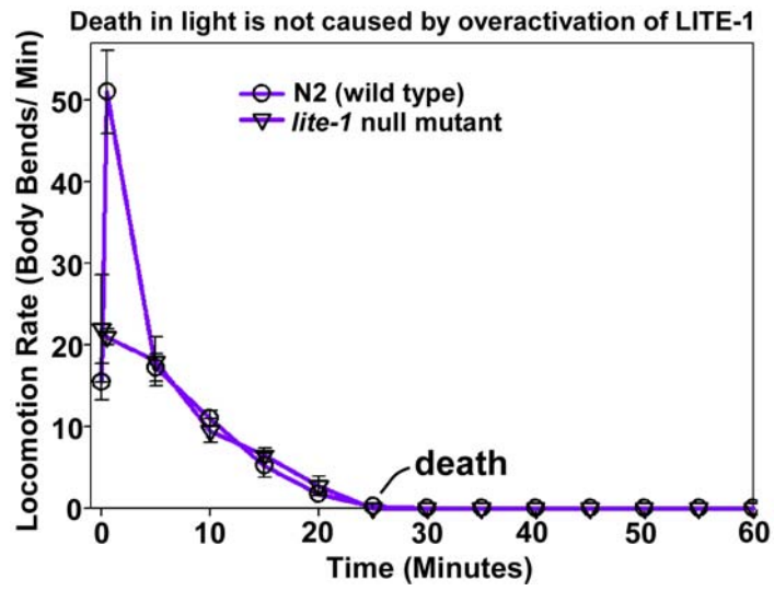
Figure S3. Death in Blue Light is Not Caused by Overactivation of LITE-1
