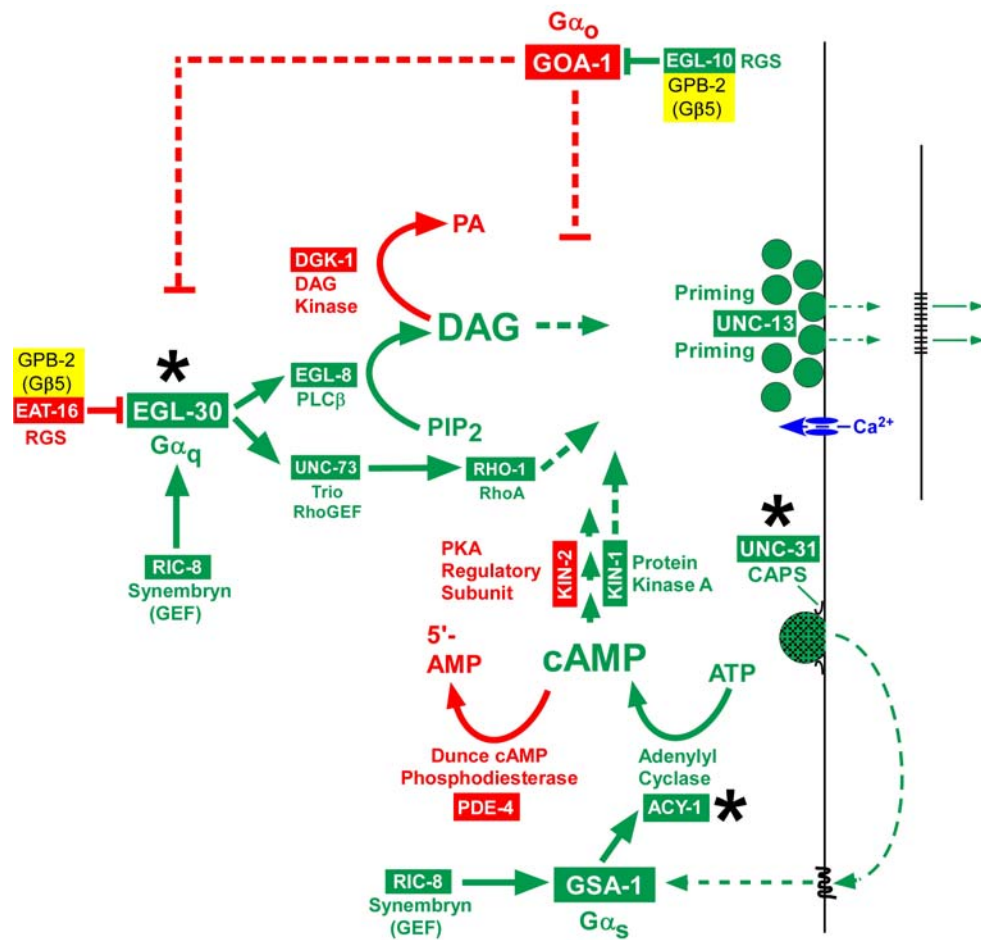
Figure S1. The Synaptic Signaling Pathways that Drive Locomotion in C. elegans
