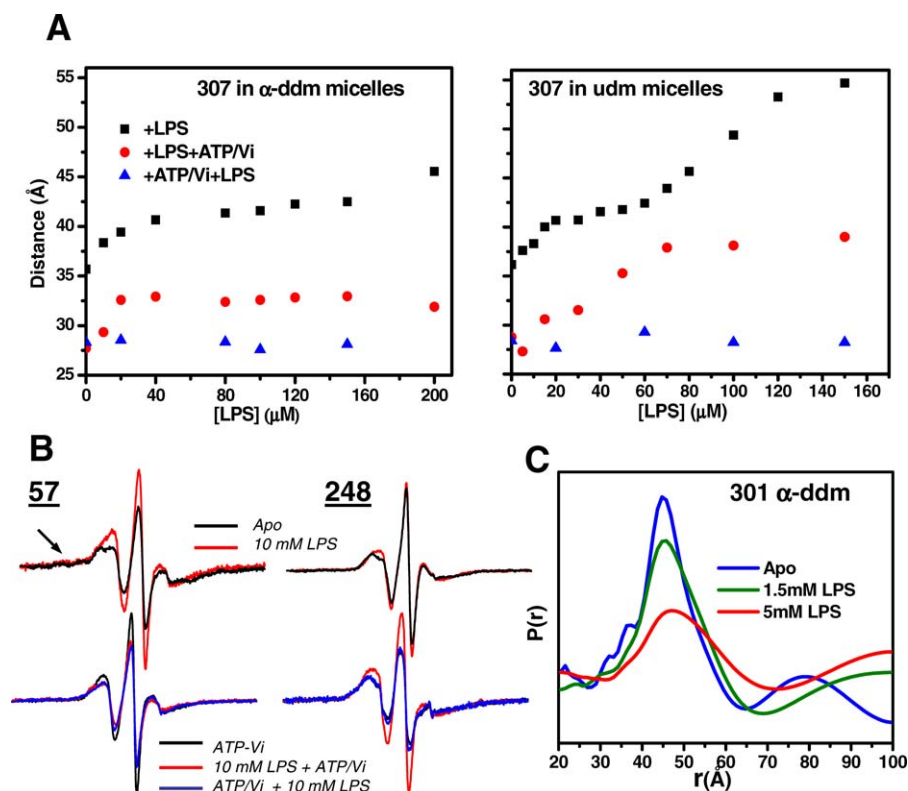
Figure 3. LPS-Induced Structural Changes in MsbA
